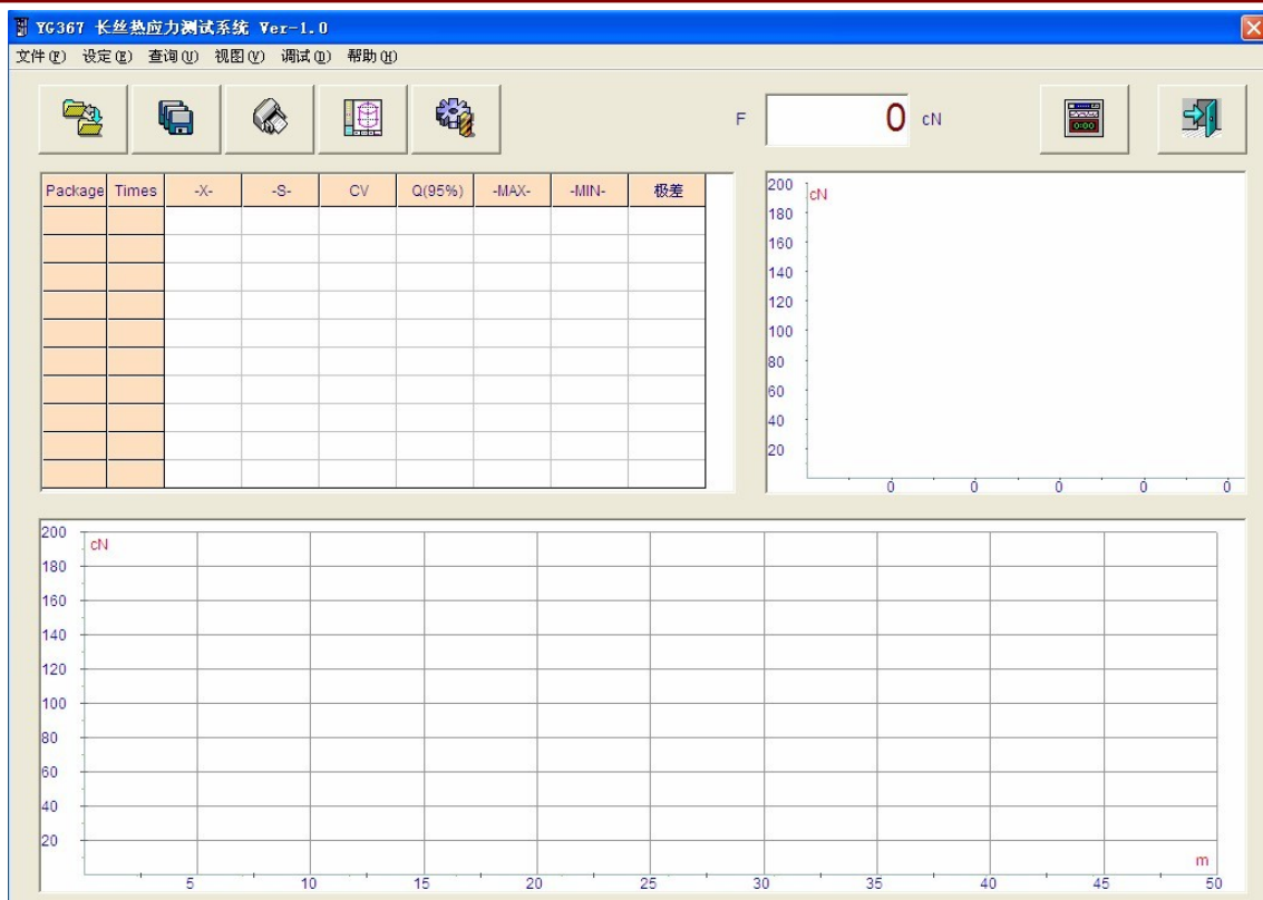
Software
